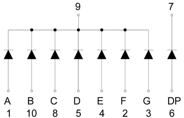
Common Cathode
