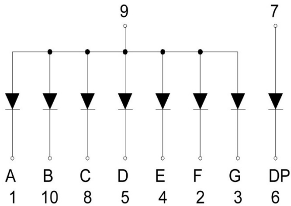
Common Anode
