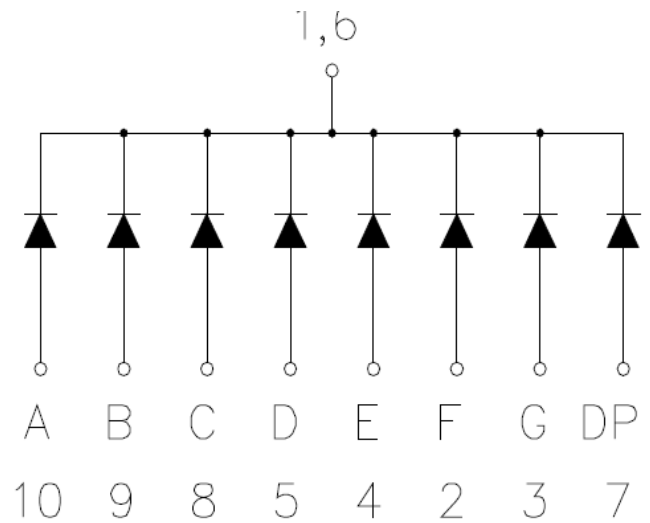
Common Cathode
