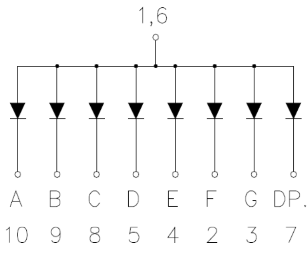
Common Anode
