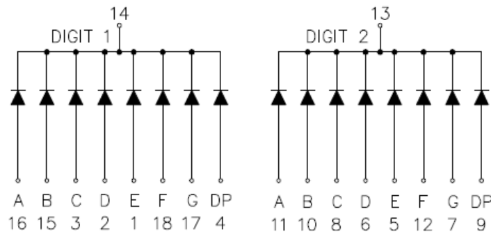
Common Cathode
