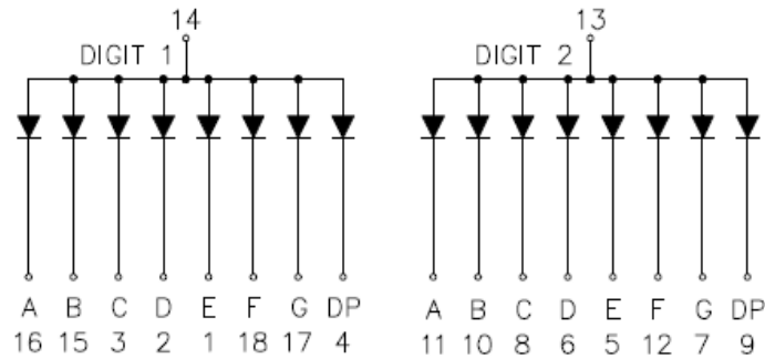
Common Anode
