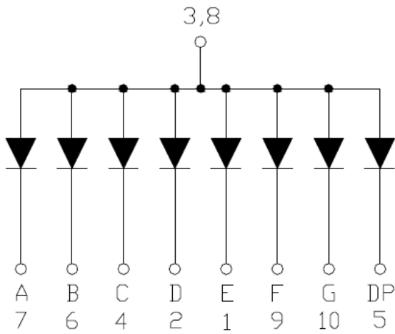
Common Anode
