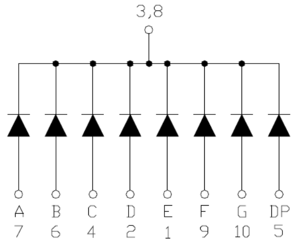
Common Cathode
