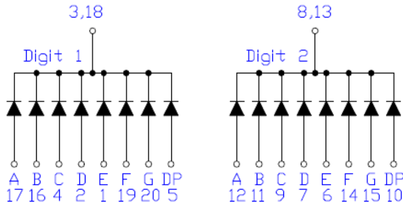
Common Cathode
