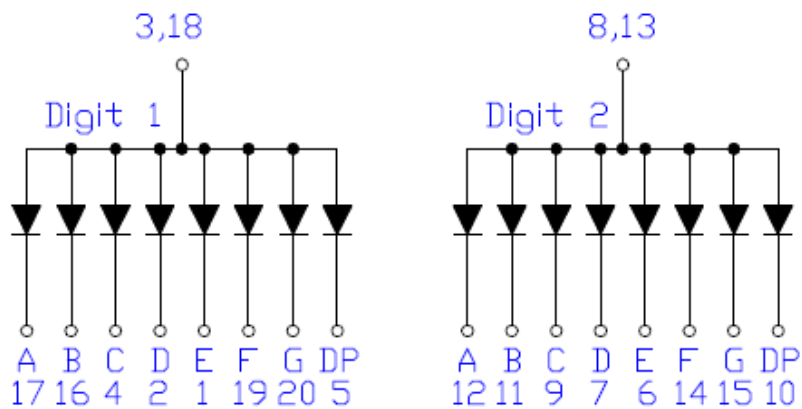
Common Anode
