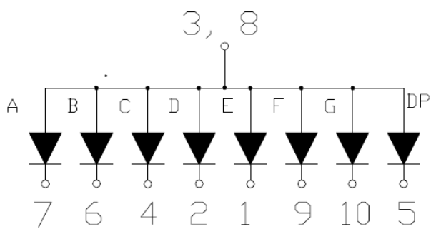
Common Anode
