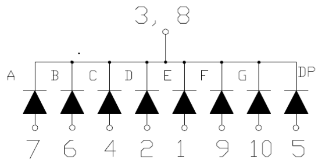
Common Cathode
