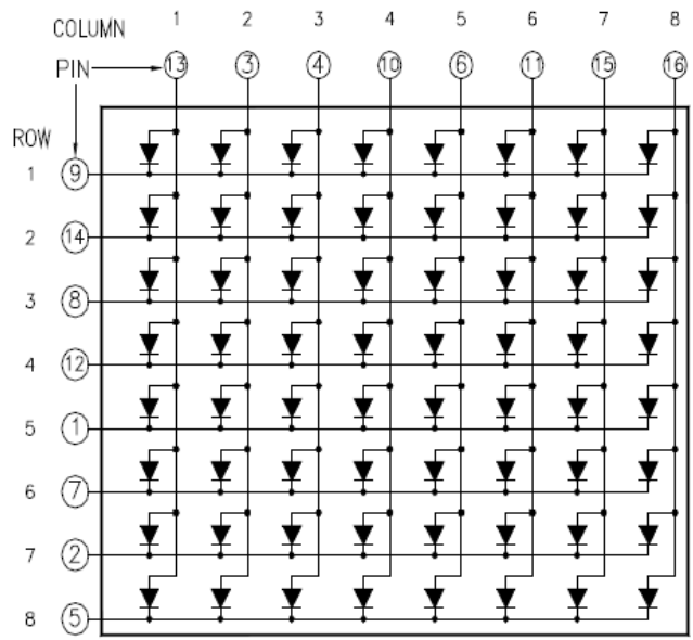
Common Column Anode
