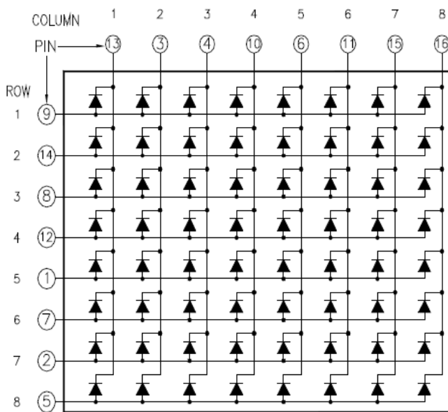
Common Column Cathode
