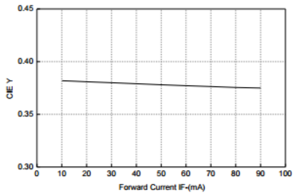
Figure5. CIE Y VS. Forward Current
