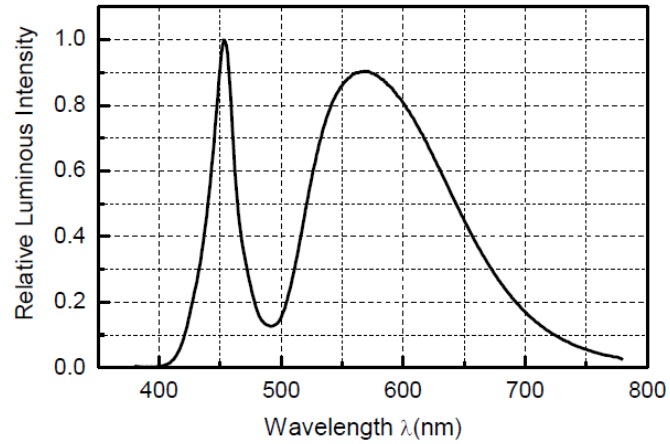
Figure7. Relative Spectral Power Distribution VS. Wavelength
