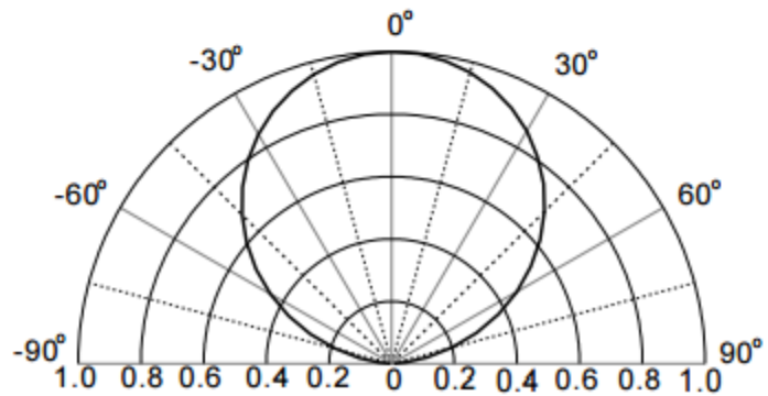
Figure6. Relative Luminosity VS. Radiation Angle
