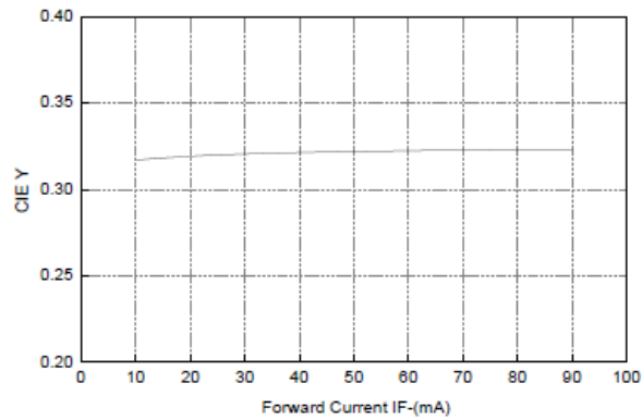
Figure5. CIE Y VS. Forward Current
