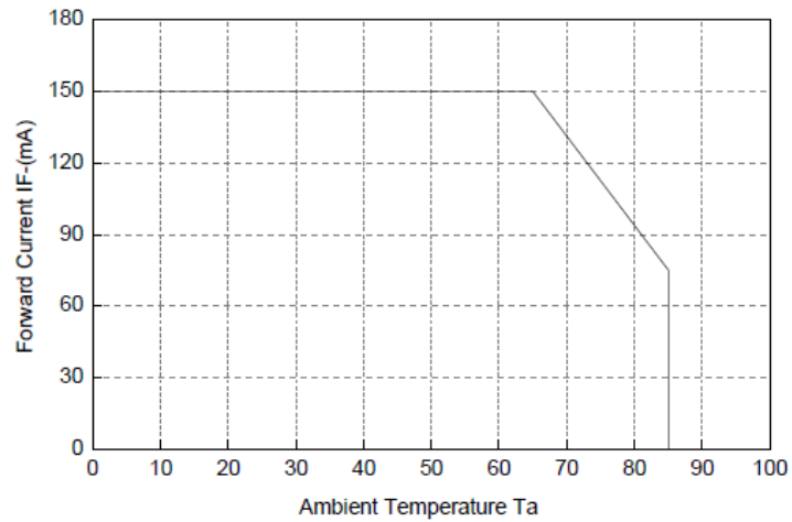
Figure1 Forward Current VS Ambient Temperature
