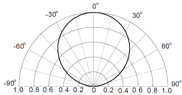
Figure6. Relative Luminosity VS. Radiation Angle
