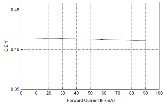
Figure5. CIE Y VS. Forward Current
