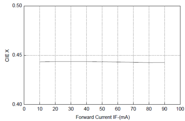
Figure4. CIE X VS. Forward Current
