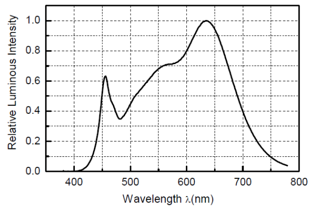
Figure7. Relative Spectral Power Distribution VS. Wavelength
