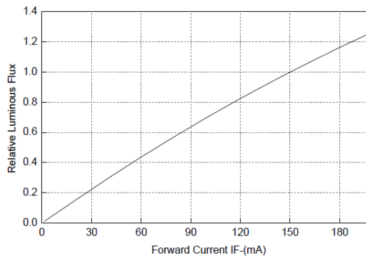
Figure3. Relative Luminous Flux VS. Forward Current
