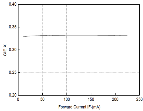
Figure4. CIE X VS. Forward Current
