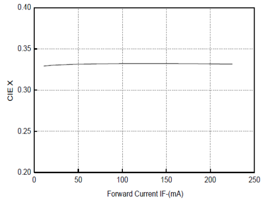
Figure4. CIE X VS. Forward Current
