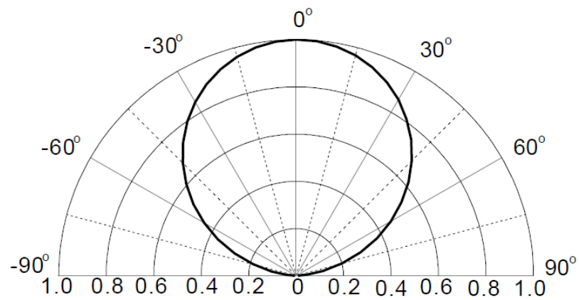
Figure6. Relative Luminosity VS. Radiation Angle
