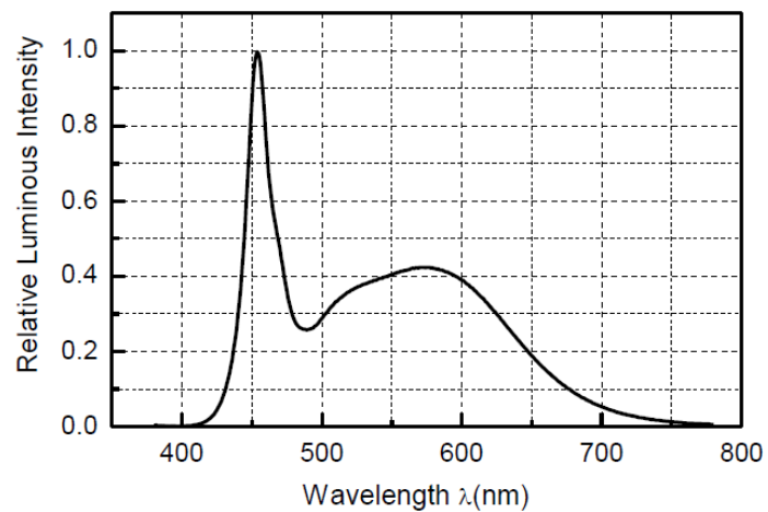
Figure7. Relative Spectral Power Distribution VS. Wavelength
