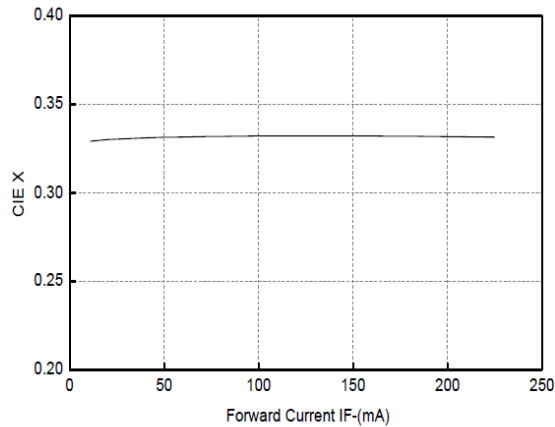
Figure4. CIE X VS. Forward Current
