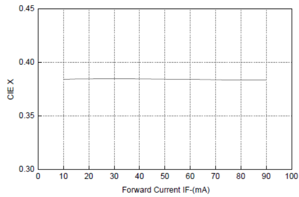
Figure4. CIE X VS. Forward Current
