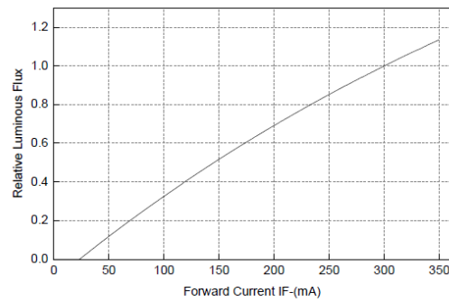
Figure3. Relative Luminous Flux VS. Forward Current
