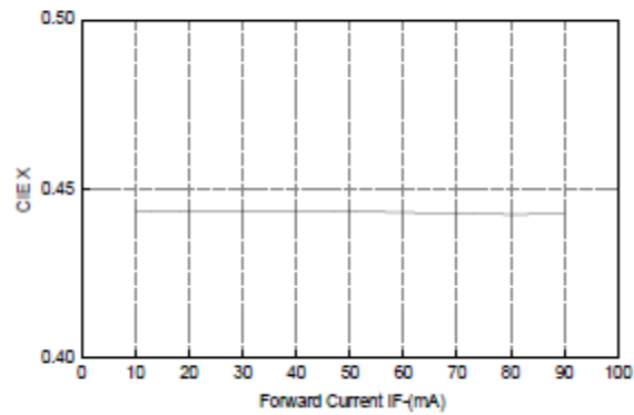
Figure4. CIE X VS. Forward Current
