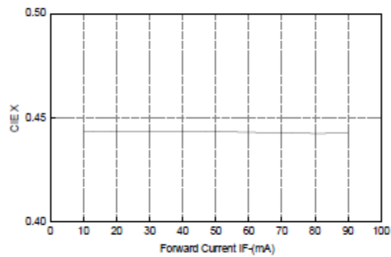
Figure4. CIE X VS. Forward Current
