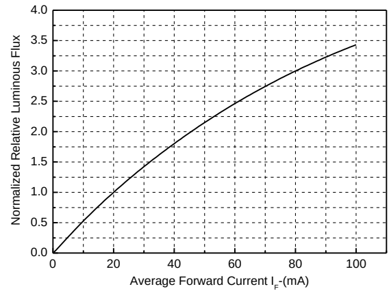
Figure2. Relative Luminous Flux VS. Forward Current
