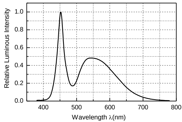
Figure4. Relative Spectral Power Distribution VS. Wavelength
