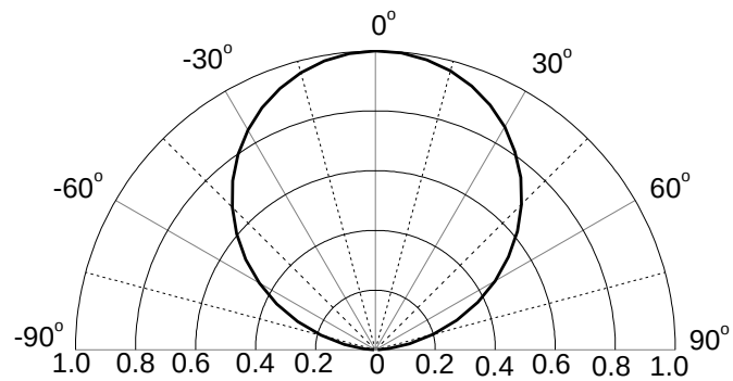
Figure5. Relative Luminosity VS. Radiation Angle
