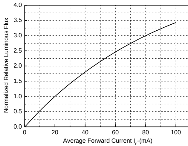
Figure2. Relative Luminous Flux VS. Forward Current
