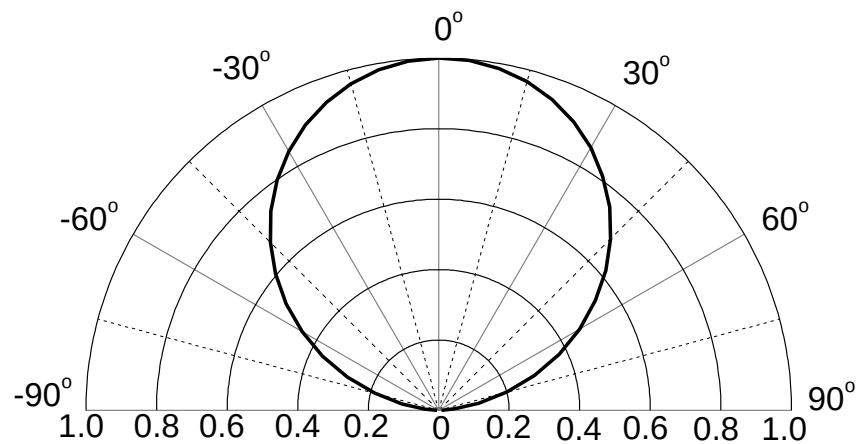
Figure5. Relative Luminosity VS. Radiation Angle
