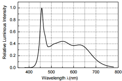
Figure3. Relative Spectral Power Distribution VS. Wavelength
