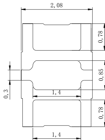
Recommended Solder Pattern
