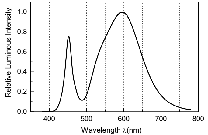
Figure2. Relative Spectral Power Distribution VS. Wavelength
