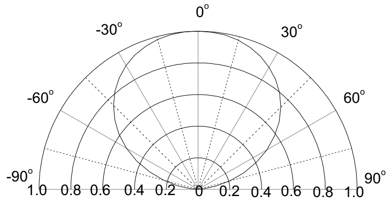
Figure3. Relative Luminosity VS. Radiation Angle
