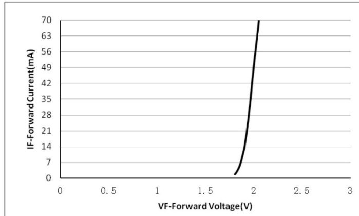
Figure1. Forward Current VS. Forward Voltage
