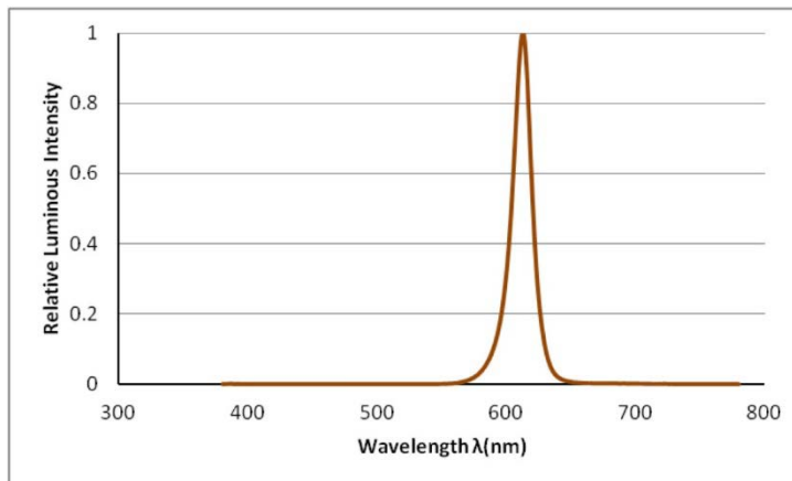
Figure2. Relative Luminous Intensity VS. Wavelength
