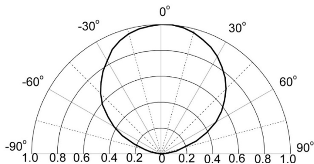
Figure3. Relative Luminosity VS. Radiation Angle
