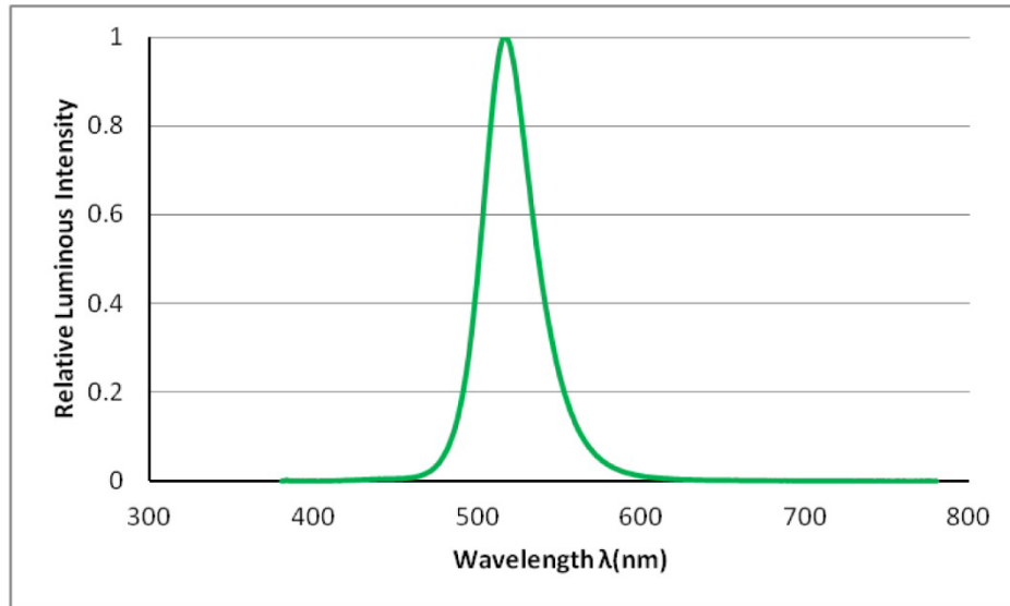
Figure3. Relative Luminous Intensity VS. Wavelength
