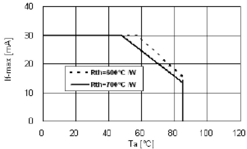
Figure2. Maximum Driving Forward DC Current VS. Ambient Temperature
