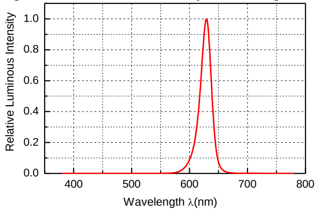
Figure3. Relative Luminous Intensity VS. Wavelength
