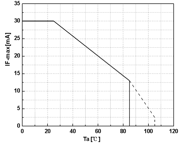
Figure2. Maximum Driving Forward DC Current VS. Ambient Temperature
