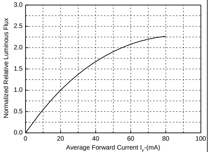
Figure2. Relative Luminous Flux VS. Forward Current
