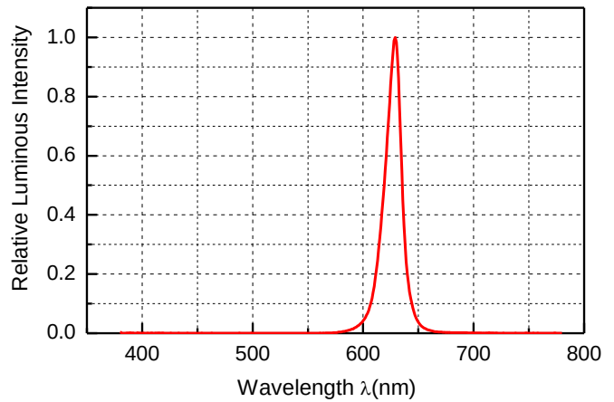
Figure4. Relative Luminous Intensity VS. Wavelength
