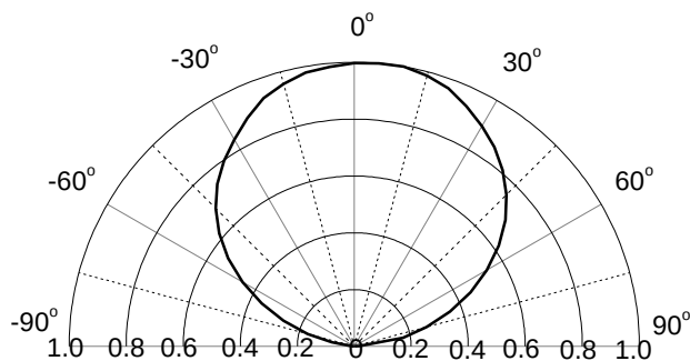
Figure5. Relative Luminosity VS. Radiation Angle
