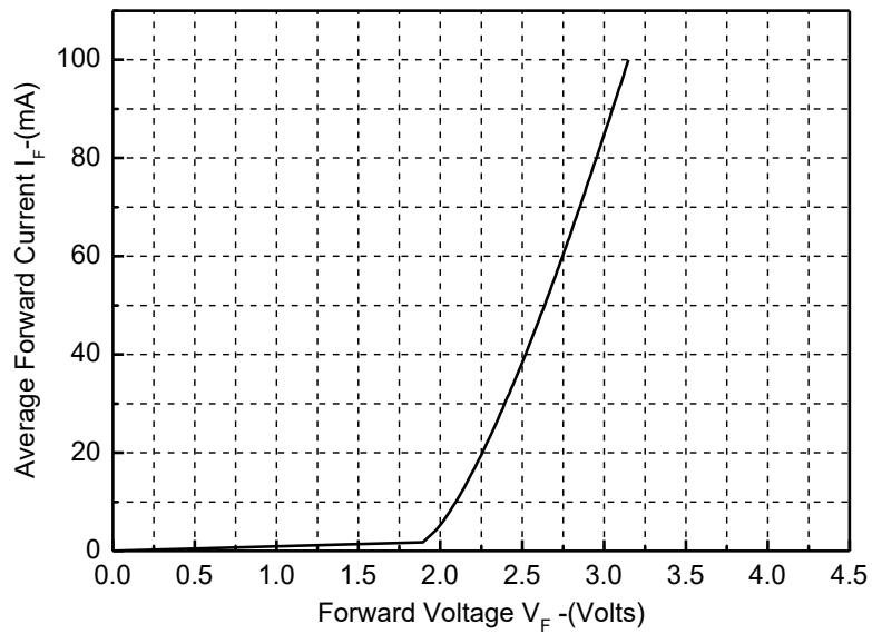
Figure1. Forward Current VS. Forward Voltage
