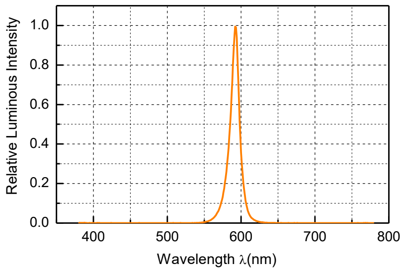
Figure2. Relative Luminous Intensity VS. Wavelength
