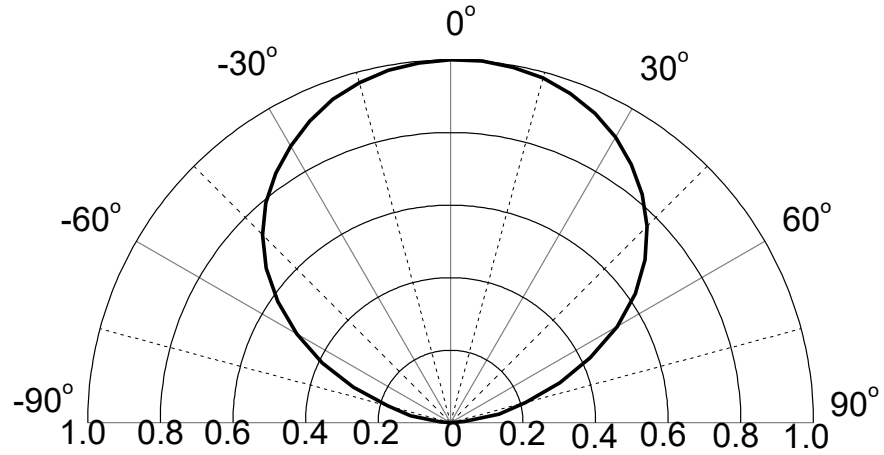
Figure3. Relative Luminosity VS. Radiation Angle
