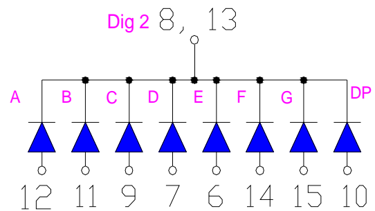
Common Cathode
