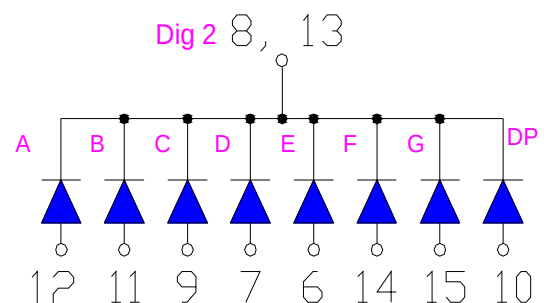
Common Cathode
