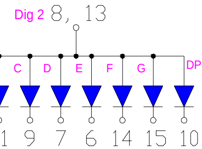
Common Anode
