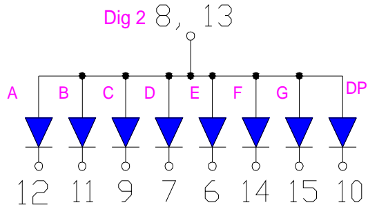
Common Anode
