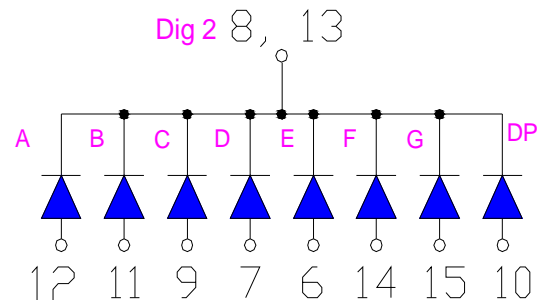
Common Cathode
