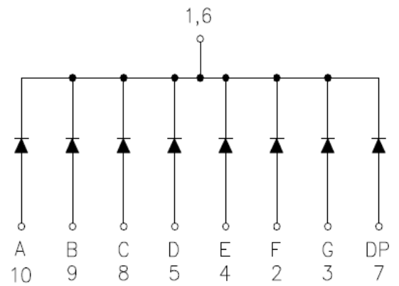
Common Cathode
