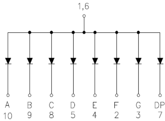
Common Anode
