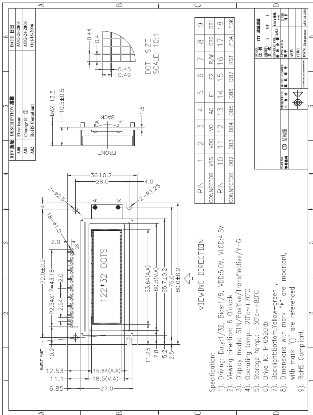
Figure 1. Dimension outline
