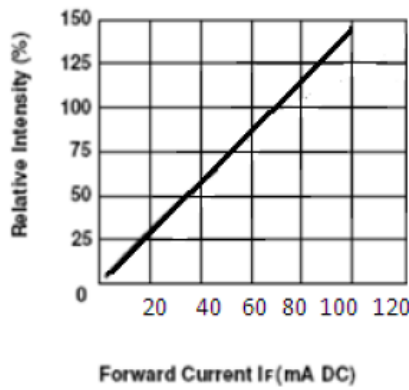
Fig 3. Relative Intensity Vs. Forward Current
