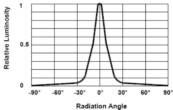
Fig 6. Radiation Diagram
