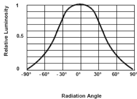
Fig 6. Radiation Diagram
