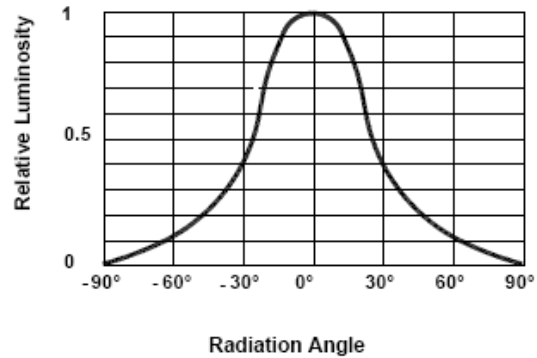
Fig 6. Radiation Diagram
