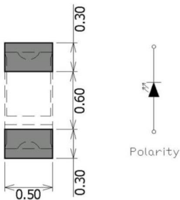
Soldering Pattern
