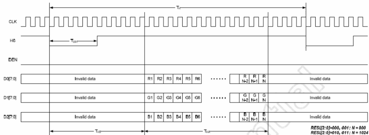
SYNC Mode Horizontal Data Format
